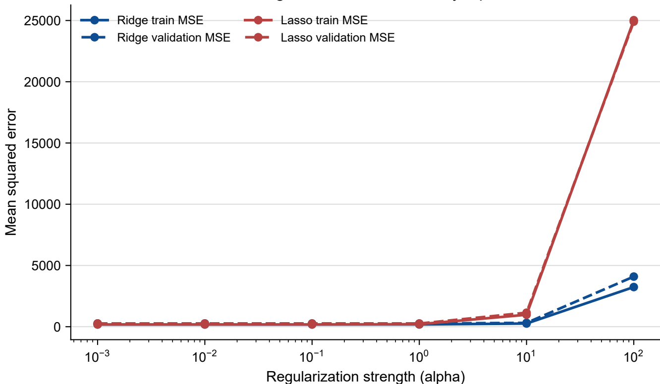
Training and validation MSE by alpha
